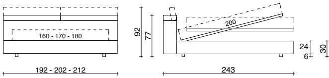
SPONDA LARGE TESTATA CON MECCANISMO BASE CONTENITORE A 1 APERTURA O A 2 POSIZIONI LARGE FRAME HEADBOARD WITH MECHANISM, SINGLE-OPENING OR DUAL-POSITION STORAGE BASE
