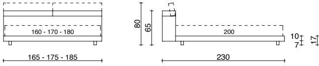
BASIC TESTATA CON MECCANISMO FASCE IMBOTTITE H. 10 CM BASIC HEADBOARD WITH MECHANISM, PADDED SURROUND H. 10 CM
