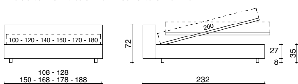
BASIC BASE CONTENITORE A 1 APERTURA O A 2 POSIZIONI BASIC SINGLE-OPENING OR DUAL-POSITION STORAGE BASE
