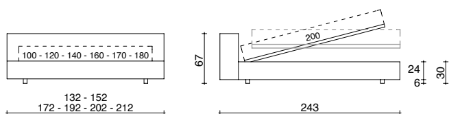
SPONDA LARGE BASE CONTENITORE A 1 APERTURA O A 2 POSIZIONI LARGE FRAME WITH SINGLE-OPENING OR DUAL-POSITION STORAGE BASE
