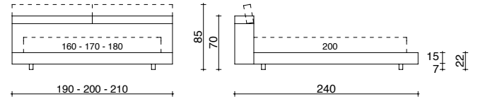
SPONDA LARGE TESTATA CON MECCANISMO FASCE IMBOTTITE H. 15 CM LARGE FRAME HEADBOARD WITH MECHANISM PADDED SURROUND H. 15 CM
