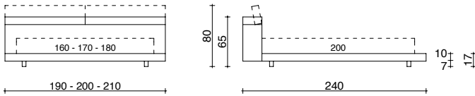
SPONDA LARGE TESTATA CON MECCANISMO BASE CONTENITORE A 1 APERTURA O A 2 POSIZIONI LARGE FRAME HEADBOARD WITH MECHANISM, SINGLE-OPENING OR DUAL-POSITION STORAGE BASE
