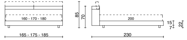
BASIC TESTATA CON MECCANISMO FASCE IMBOTTITE H. 15 CM BASIC HEADBOARD WITH MECHANISM, PADDED SURROUND H. 15 CM
