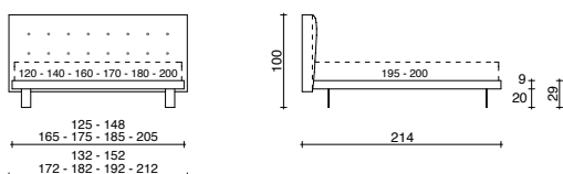
BASIC FASCE IMBOTTITE H. 9 CM BASIC PADDED SURROUND H. 9 CM
