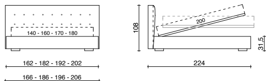
SPONDA LARGE BASE CONTENITORE A 1 APERTURA O A 2 POSIZIONI LARGE FRAME SINGLE-OPENING OR DUAL-POSITION STORAGE BASE
