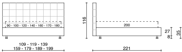
SPONDA LARGE ALTO TESTATA TRAPUNTATA H. 116 CM FASCE IMBOTTITE H. 27 CM LARGE FRAME TALL QUILTED HEADBOARD H. 116 CM, PADDED SURROUND H. 27 CM
