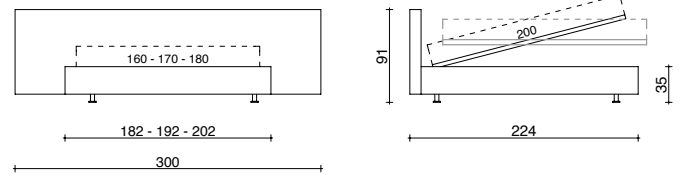
LONG SPONDA LARGE H. 91 CM BASE CONTENITORE A 1 APERTURA O A 2 POSIZIONI LONG FRAME LARGE H. 91 CM WITH SINGLE-OPENING OR DUAL-POSITION STORAGE BASE
