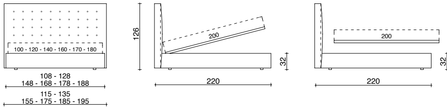
BASE CONTENITORE STORAGE BASE
