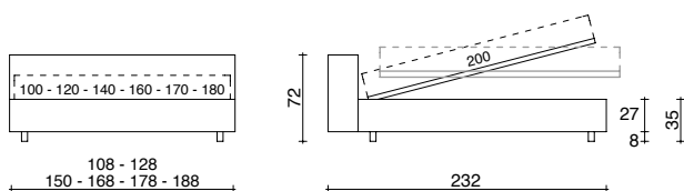
BASIC BASE CONTENITORE A 1 APERTURA O A 2 POSIZIONI BASIC SINGLE-OPENING OR DUAL-POSITION STORAGE BASE
