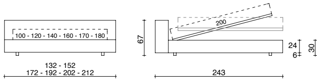
SPONDA LARGE BASE CONTENITORE A 1 APERTURA O A 2 POSIZIONI LARGE FRAME WITH SINGLE-OPENING OR DUAL-OPENING STORAGE BASE
